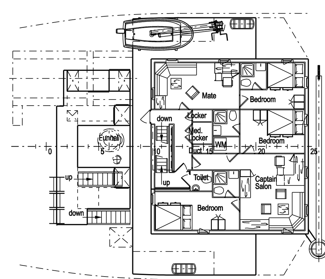
CAPTAINSDECK
