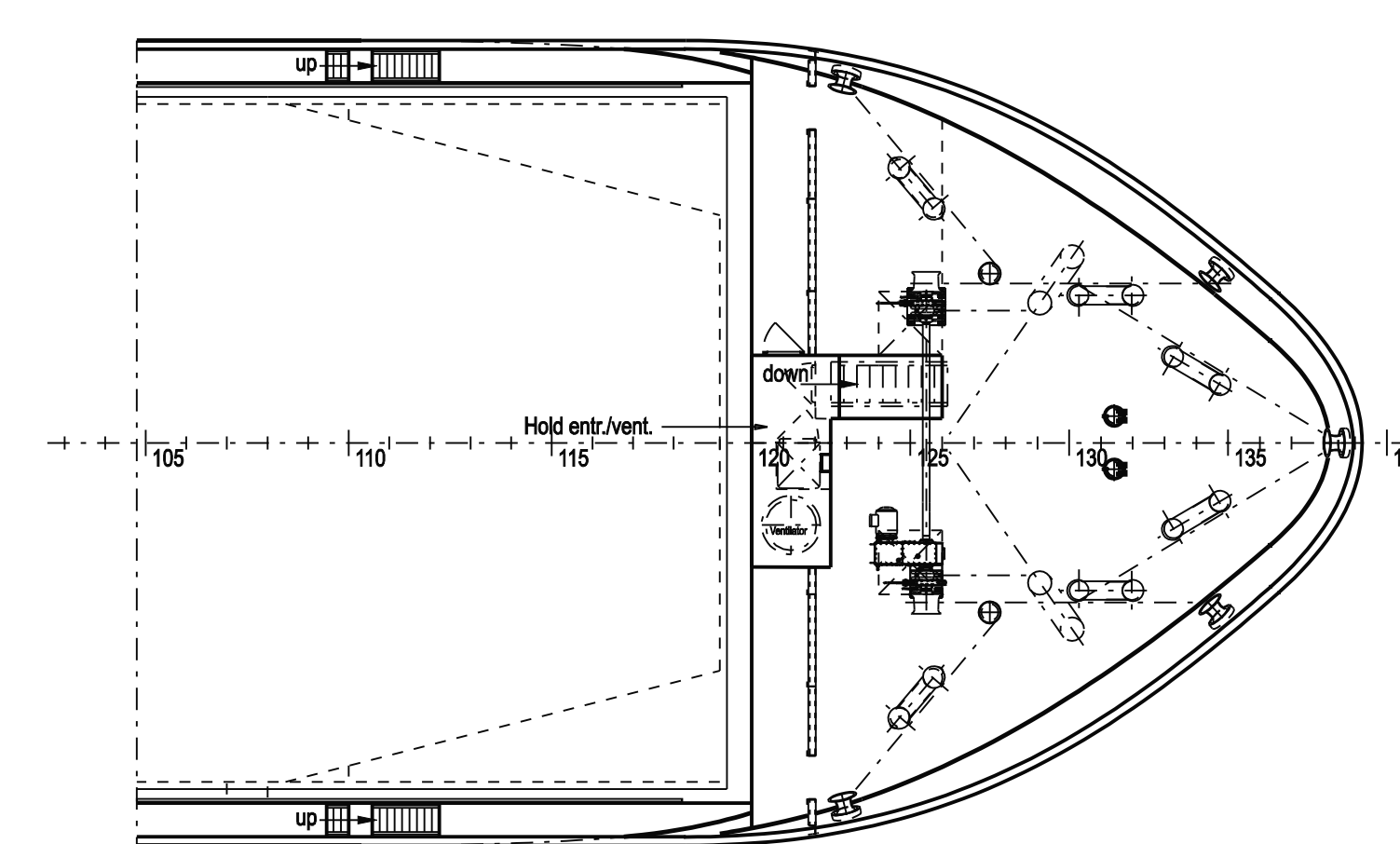
FORECASTLEDECK
