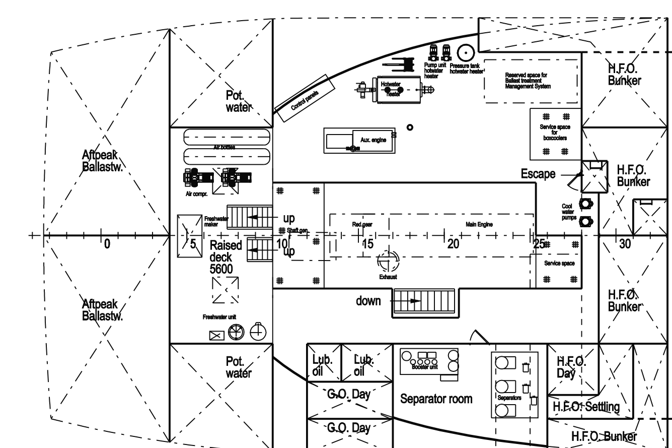
TWEENDECK AFT.
